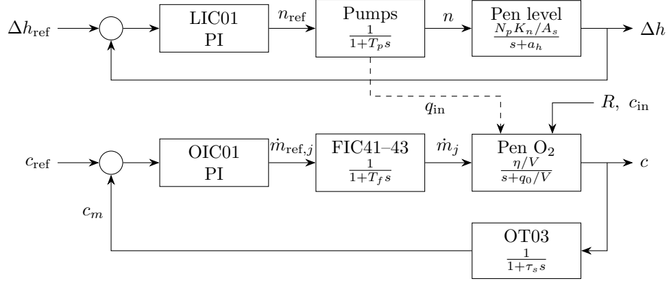
Figure 1: Control structure. The dashed line is the coupling from pump flow to oxygen.
